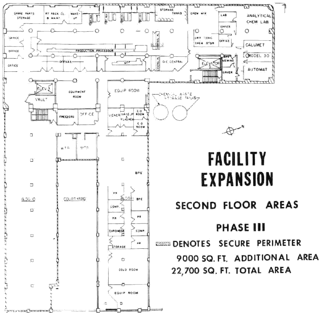
Figure 8-3. Facility Expansion, Phase III
