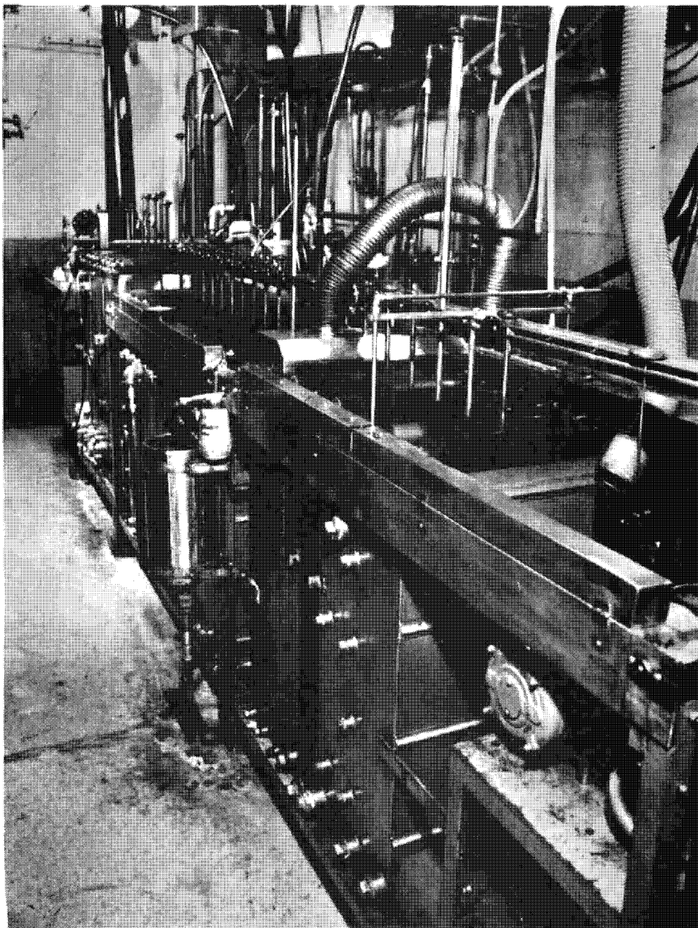
Figure 6-5. Ragdoll Processor
